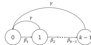
Figure 1: The multi-state model with k states.
