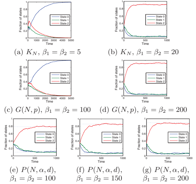
Figure 3: The dynamics of fractions x_0, x_1 and x_2 of states over time where N = 1,000 and \gamma = 1 . For the cases (ii) and (iii), p = 0.05 , \alpha = 3 and d = 50 .
