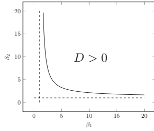
Figure 2: The phase transition diagram for the ternary model when \gamma = 1 .
